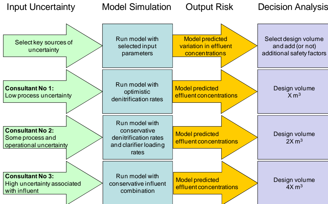
Figure 1 – Model-based design process for the three proposed solutions.
