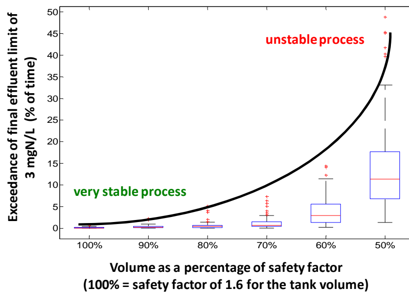
Figure 2 – Exceedance of nitrogen effluent limit as percentage of time over a 1-year evaluation period for a given process and a given time-varying influent as a function of tank size; 100% of volume refers to a design volume resulting from conservative guidelines).
